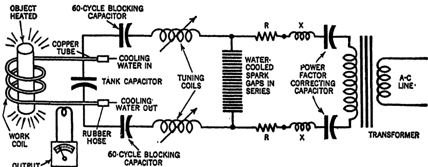
Basic spark-type high-frequency generator for induction heating of metals.
